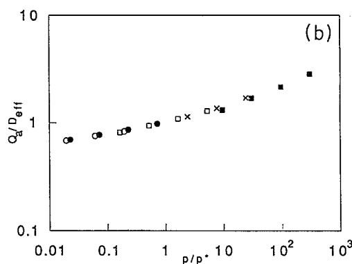
FIG. 6. Reaction rate Q_a for a poisoned 2D lattice at concentrations higher than c_0 : empty circles, c = 0.95 ; solid circles, c = 0.85 ; empty squares, c = 0.75 , Xc = 0.70 ; solid circles, c = 0.65 . (a) Reaction rate versus desorption probability. Full lines are guides to the eyes. (b) Scaled reaction rate versus scaled desorption probability.
